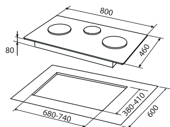
GAS HOB / FH-GS2130 GLBK
