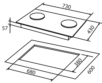
ELECTRIC HOB / FH-IC7020
