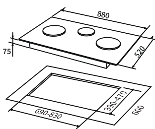
GAS HOB / FH-GS7130 FGBK
