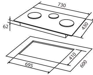
ELECTRIC HOB / FH-IC7030
