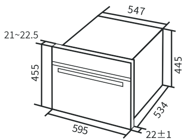
ALL-IN-ONE OVEN / FV-AL81
