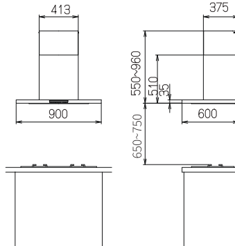
HOOD / FR-SC2090 V
