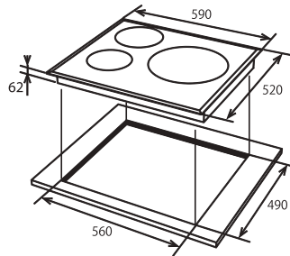
ELECTRIC HOB / FH-ID5230
