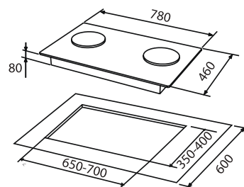
GAS HOB / FH-GS2120 GLBK
